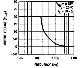
Output Voltage vs Frequency
