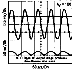
Sine Wave Response
