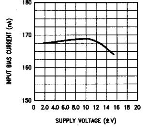
Input Bias Current vs Supply Voltage
